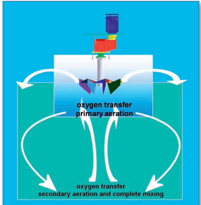
LANDY axial flow low speed surface aerators
